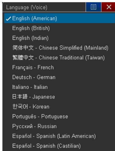
Figure 38. Language list.
