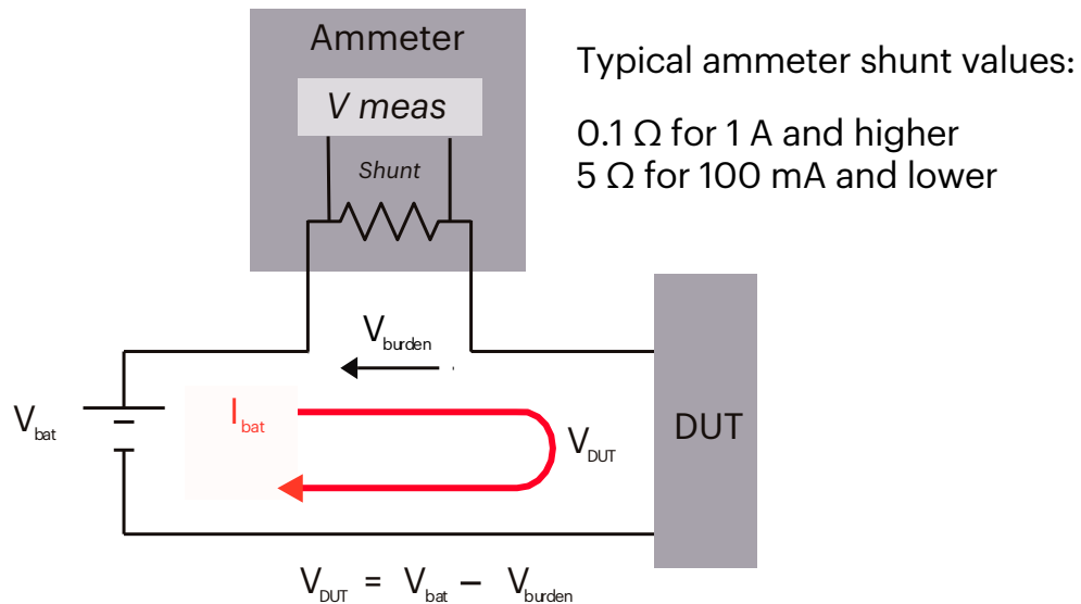
Figure 2. DMM presents burden voltage when measuring current
