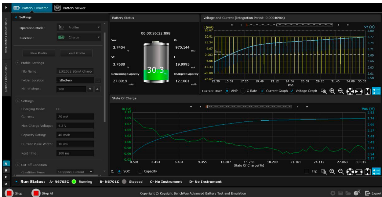
Figure 4. BV9210B creating a battery model
