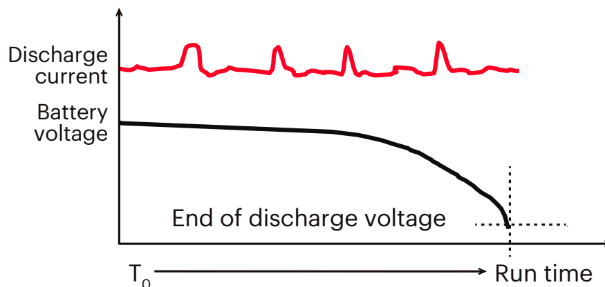
Figure 1. Battery run-down test results
