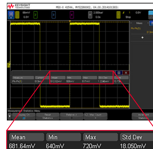
Increasing the voltage-per-division scaling
