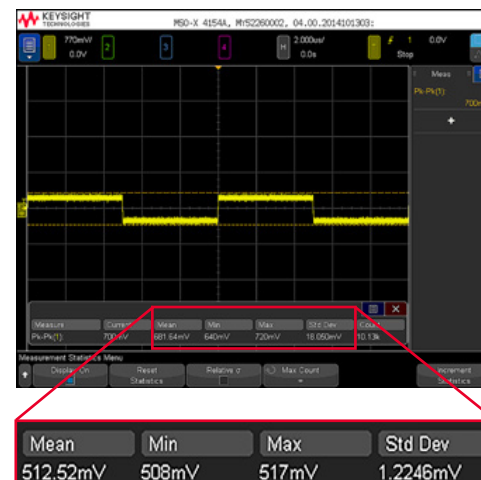
100 KHz clock signal
